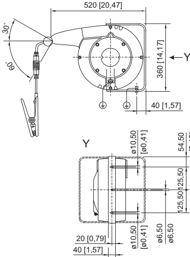
Grounding clamp with automatic retractor for cable Item no. 247671
