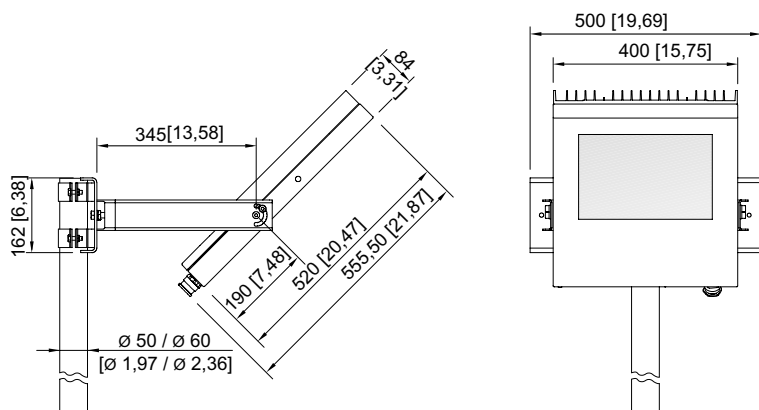
Floodlight with pole mounting
