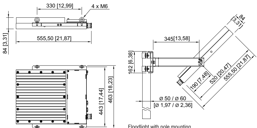
Floodlight with cooling element, with ring eyes
