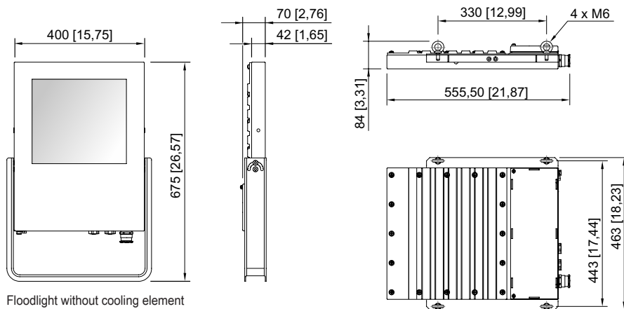
Floodlight without cooling element, with ring eyes
