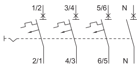
3-pole + N, without auxiliary contact
