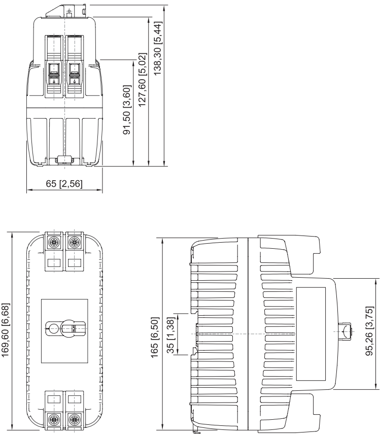
8530/1; 2 horizontal pitches
